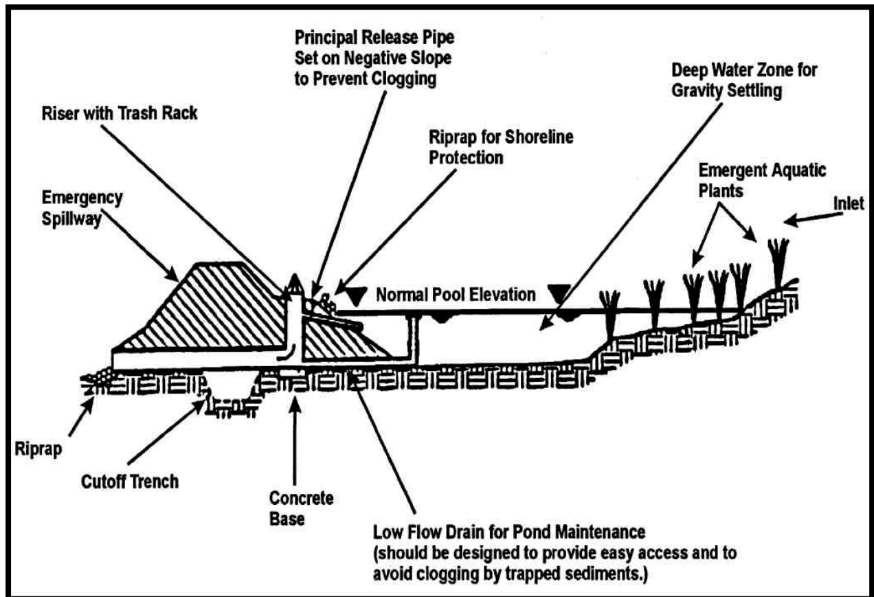
Figure 6.6-9: Typical Wet Pond Design
