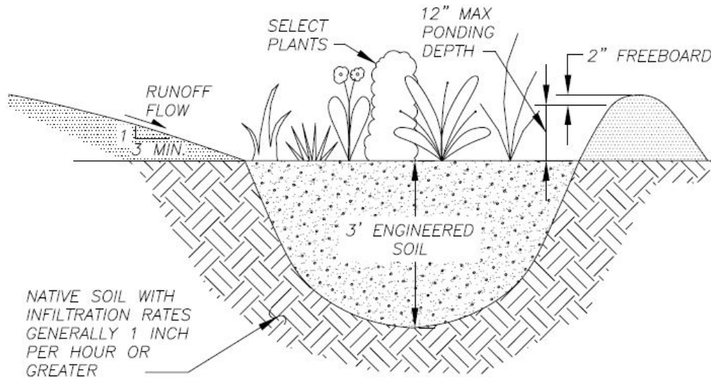
a - Standard Bioretention Profile
