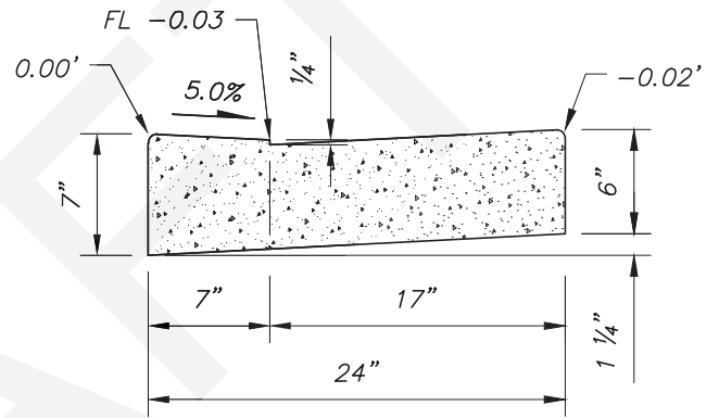
TYPE 4 (USED AT CURB CUTS)
