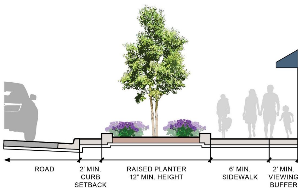
Figure 3 - 4: Urban Center Street - Raised Planter
