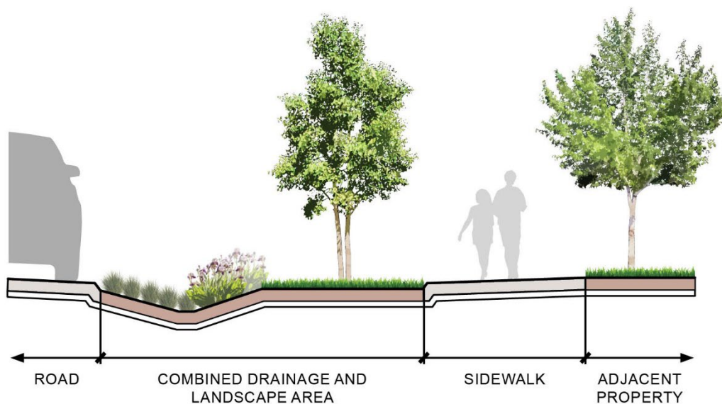
Figure 3 - 11: Rural Minor Arterial - Landscape Buffer
