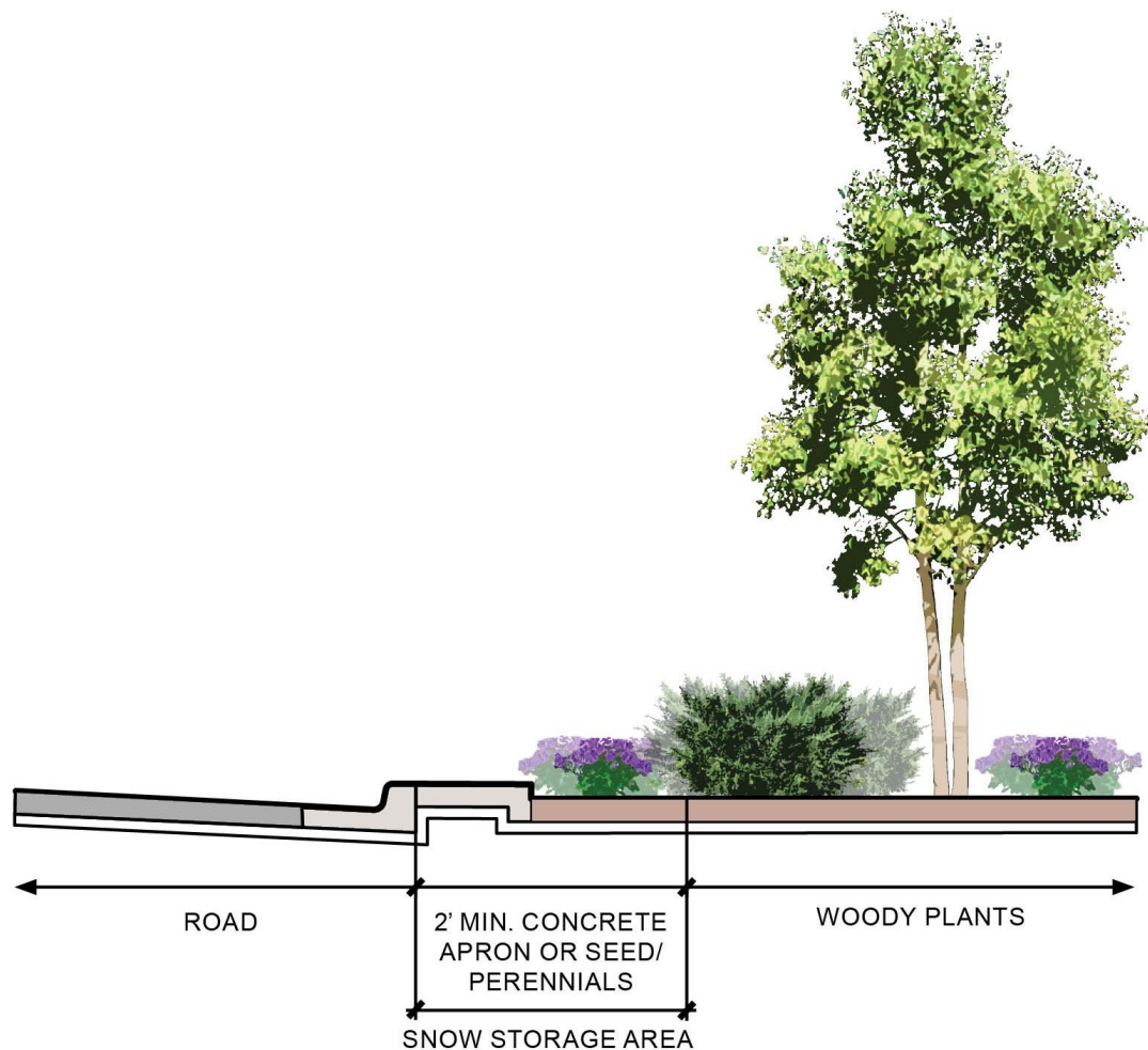
Figure 3 - 2: Snow Storage Area Without Cluster Planting
