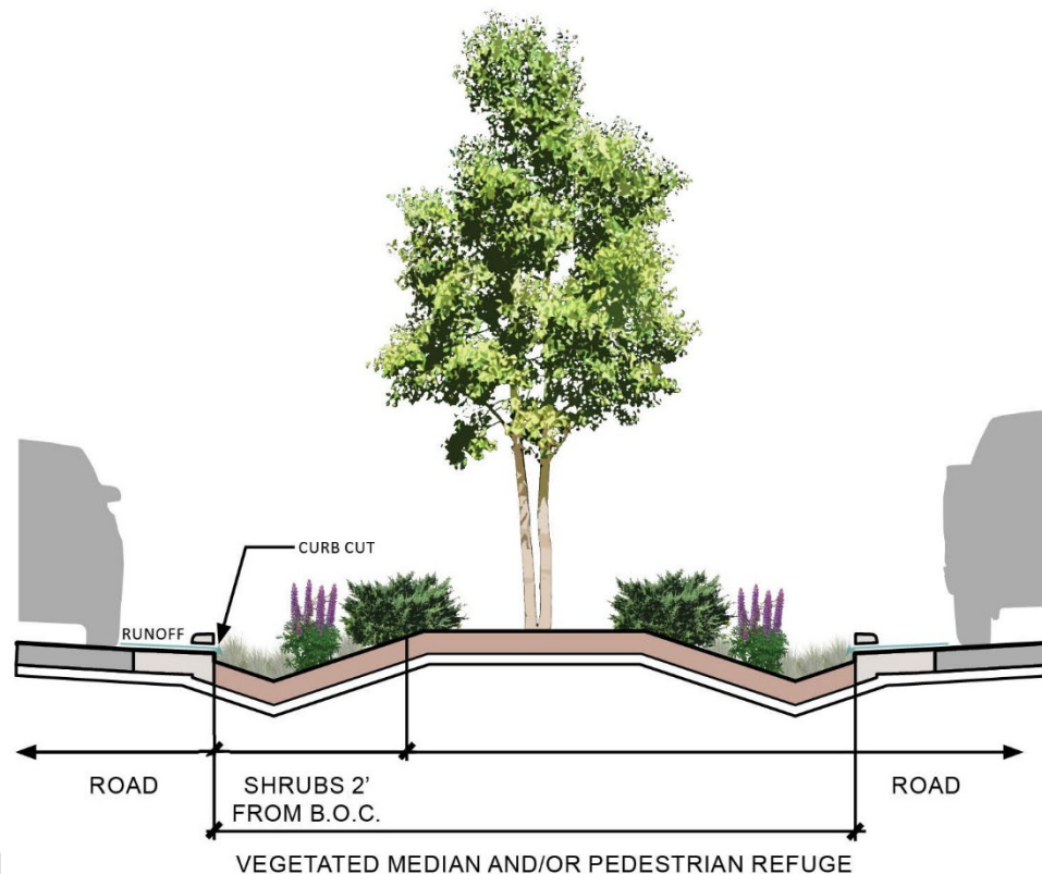
Figure 3 - 7: Urban Major Street Arterial – Median
