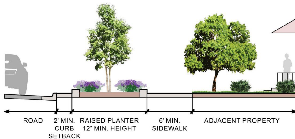
Figure 3 - 5: Urban Center Street - Residential
