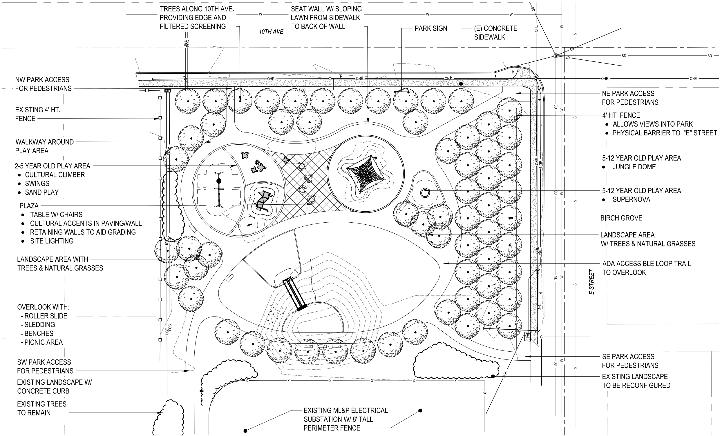
1 PLAY EQUIPMENT CONFIGURATION SCALE: 1"=20'
