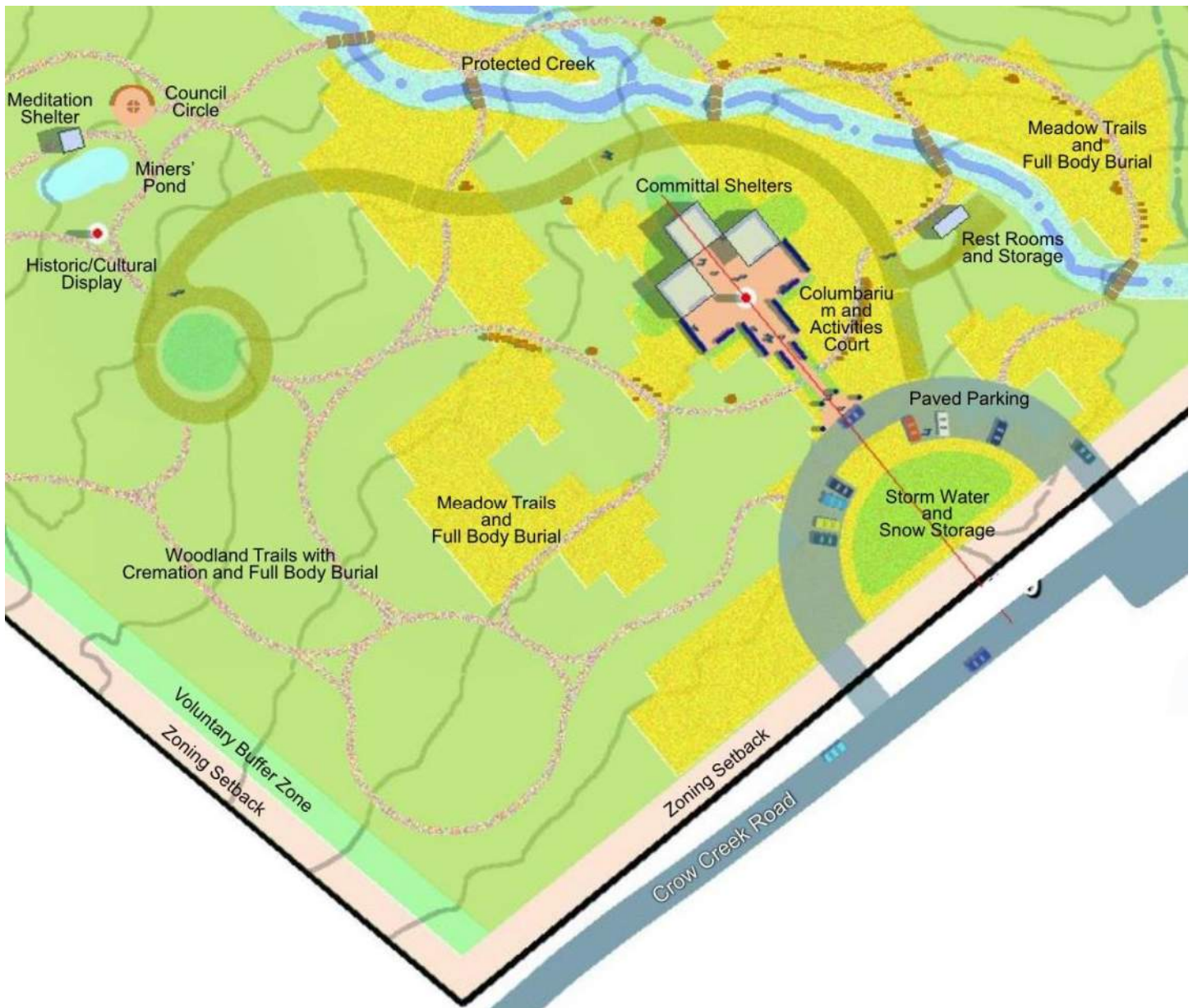
Figure 8 – Girdwood Cemetery Master Plan – Central Area and Parking
