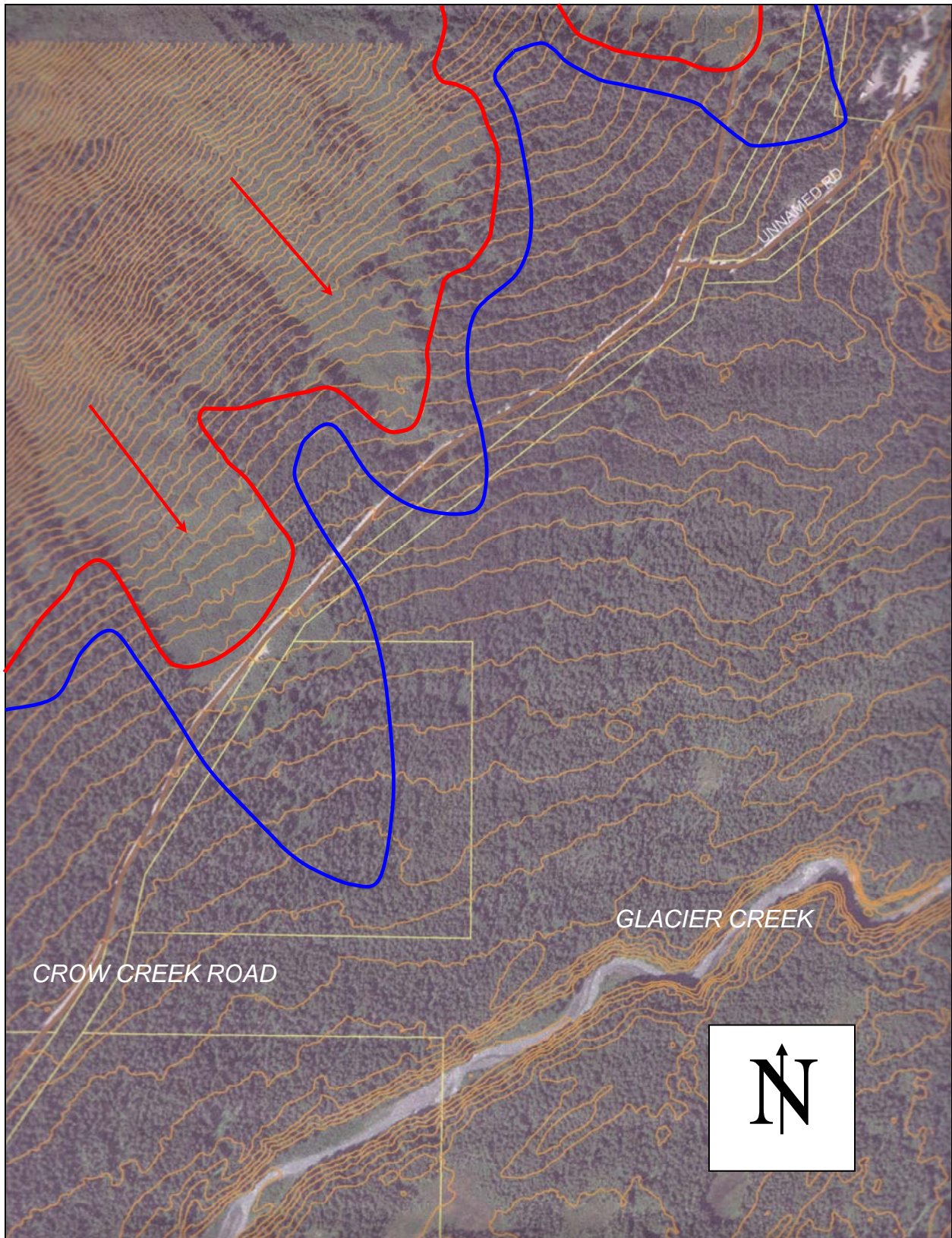
Figure 6: Avalanche Risk Along Crow Creek Road: This map delineates the limits of high (red) and moderate (blue) snow avalanche hazard affecting potential development along Crow Creek Road. The blue lines represent the design magnitude avalanche limits (>30 years, but <300 years) of the moderate hazard zone. Red lines delineate the limits of high hazard zones with return intervals <30 years. (Mapped 2-6-07 by D. Fesler, AMSC. Source map: provided by MOA/ITD, created 1-07 by Warren Elkins.)
