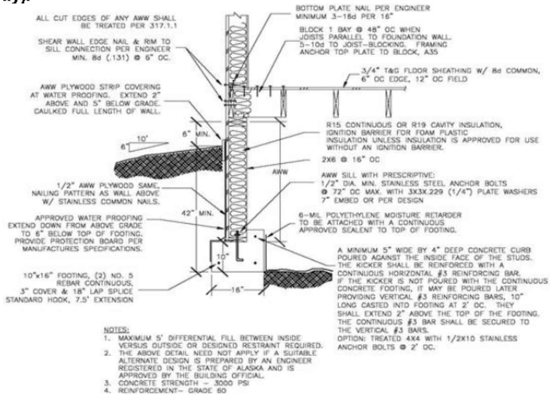
23.85. Figure R403-34 All weather wood foundation (For use in repairs only).
