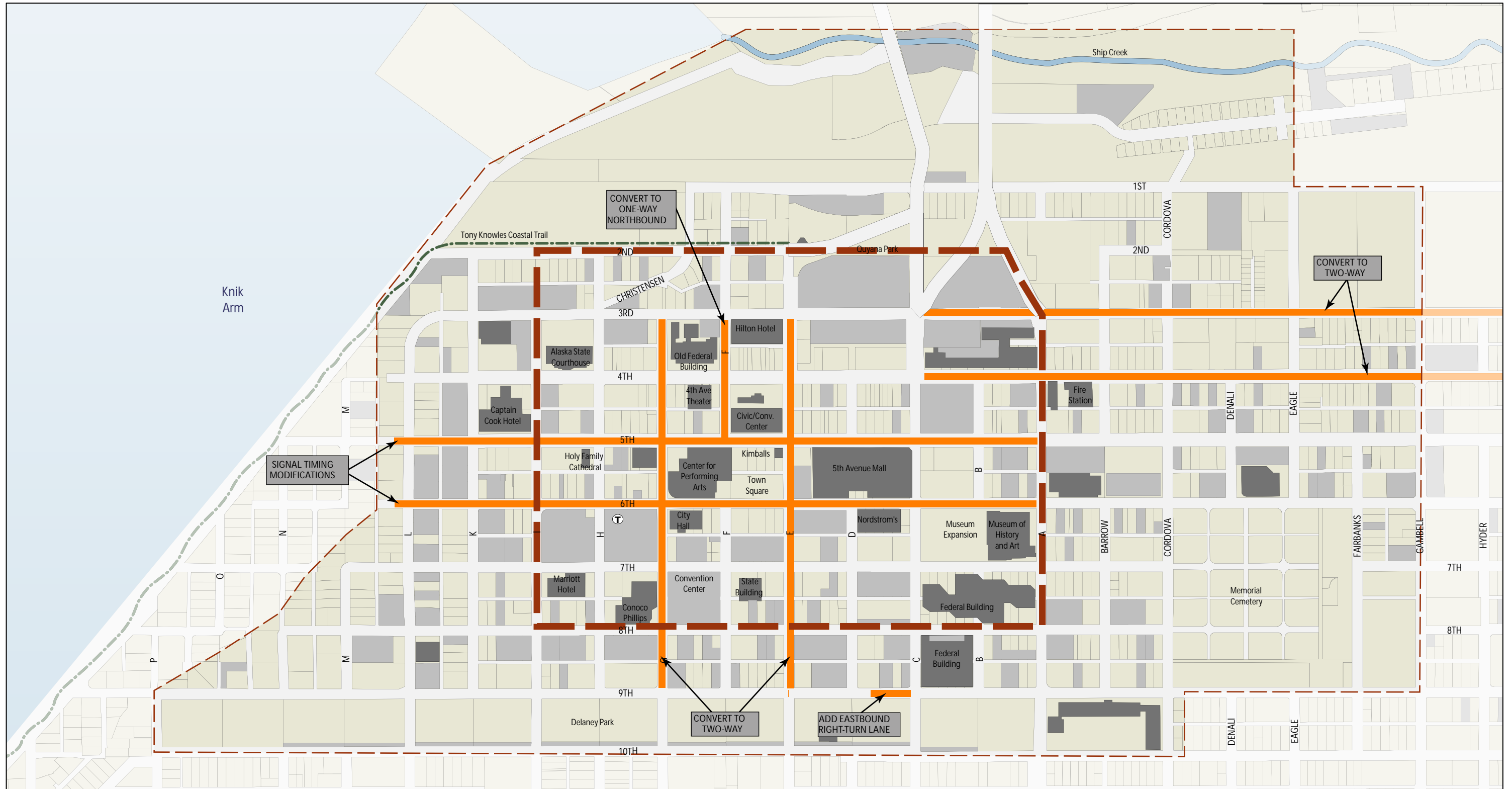
Diagram 5.3 Possible Roadway Improvements
