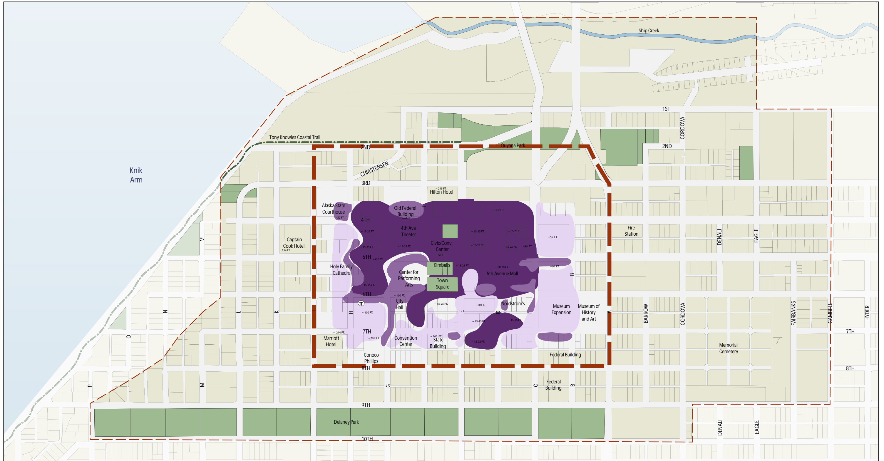
Diagram 4.1 Pedestrian Activity
