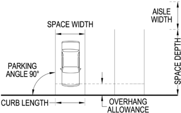
90° PARKING SPACES
