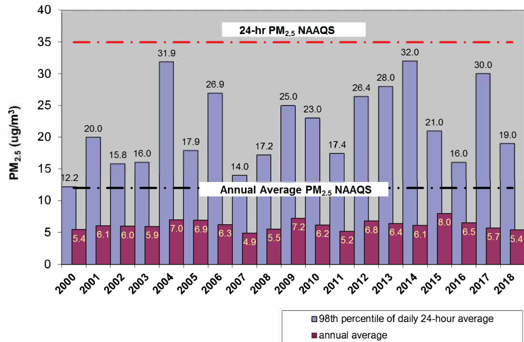
Figure 9-8 Variability of PM 2.5 , Annual Average and Yearly Maximum 24-Hr Average
