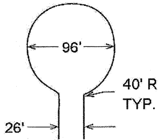
96' DIAMETER CUL-DE-SAC
