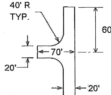
ACCEPTABLE ALTERNATIVE TO 120' HAMMERHEAD
