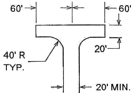
120' HAMMERHEAD
