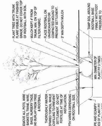
DECIDUOUS TREE PLANTING 1 L4 NTS
