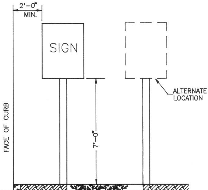
Sign Placement Curb With Sidewalk and Parkway
