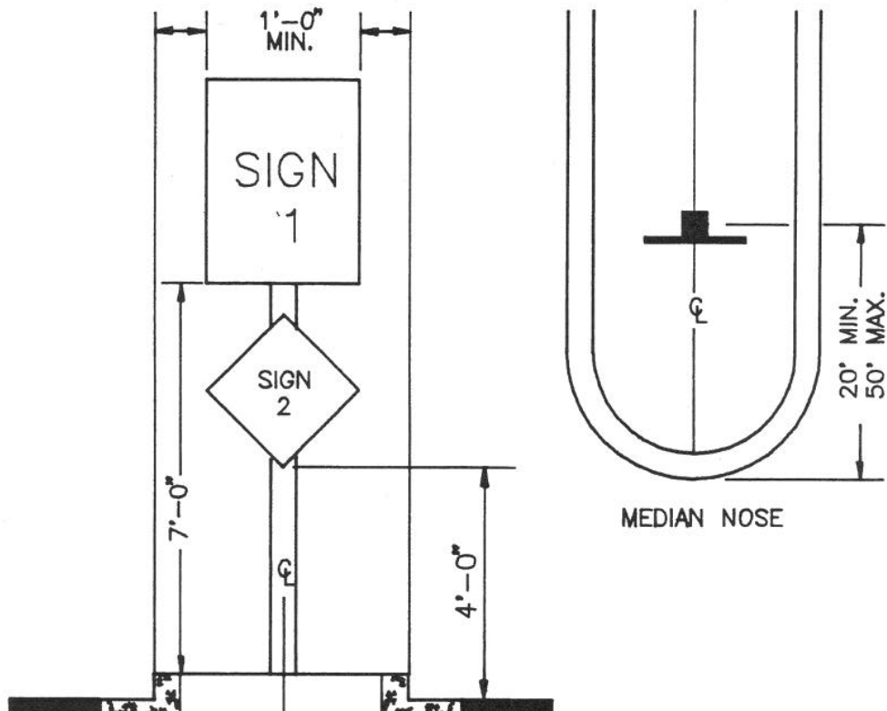
Sign Placement Medians
