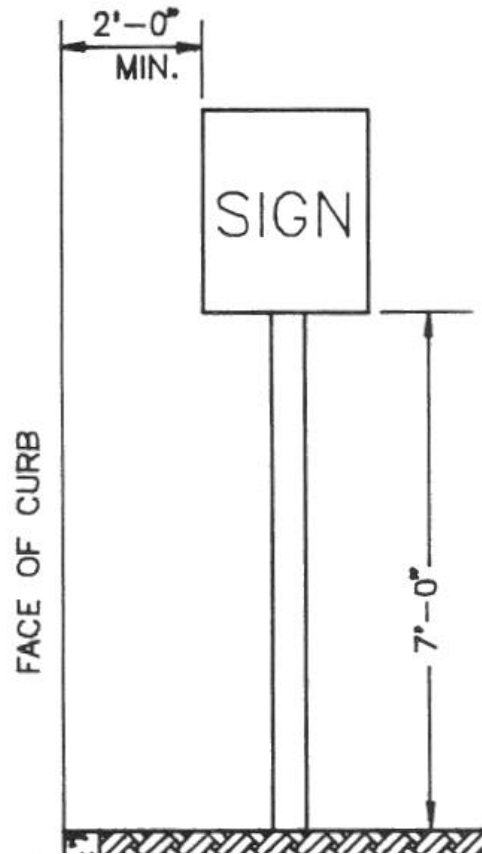
Sign Placement Curb With Sidewalk
