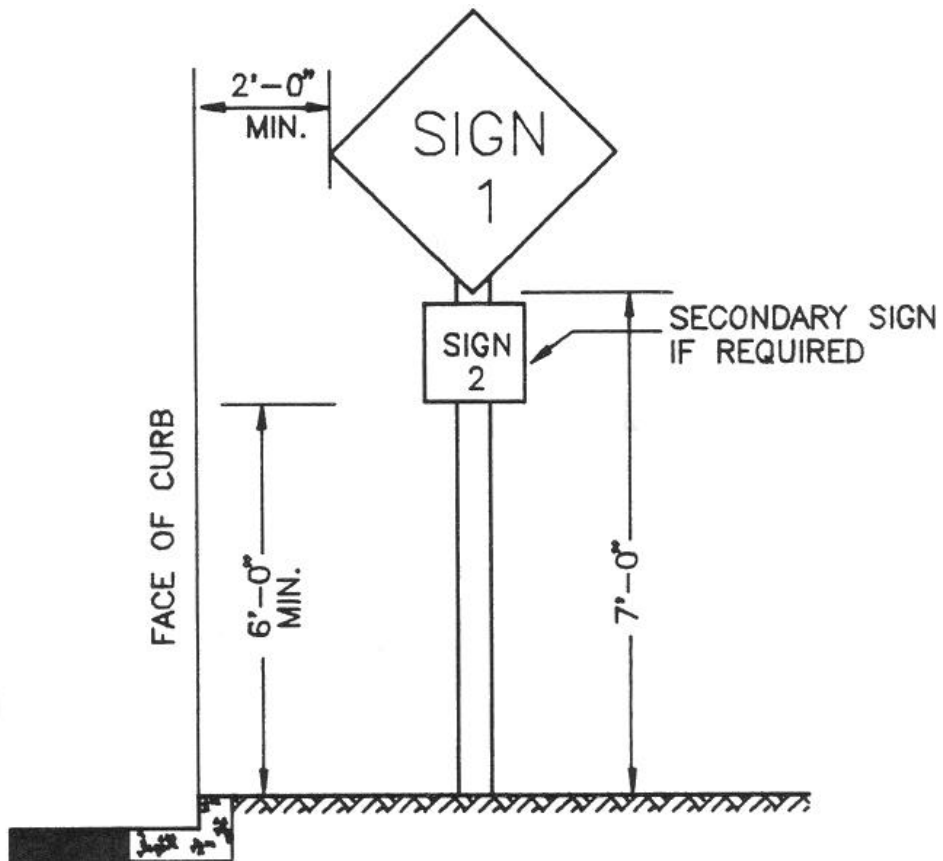
Sign Placement Curb Without Sidewalk
